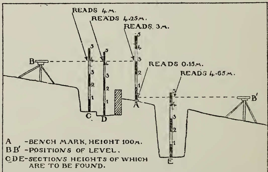
Fig. 4. The use of the Dumpy Level.
